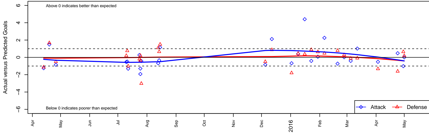
Crossfire Select Wilkinson G98 Dots are actual minus expected GF (blue circles) and GA (red triangles). Blue line is smoothed change in attack strength. Red is smoothed change in defense strength.
